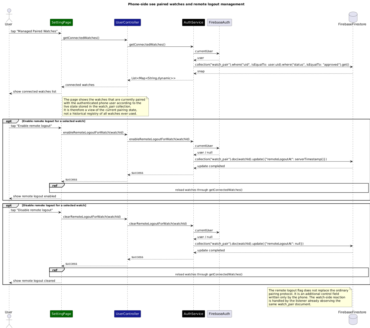
Figure 2.11: Phone-side view paired watches and remote logout management sequence diagram
