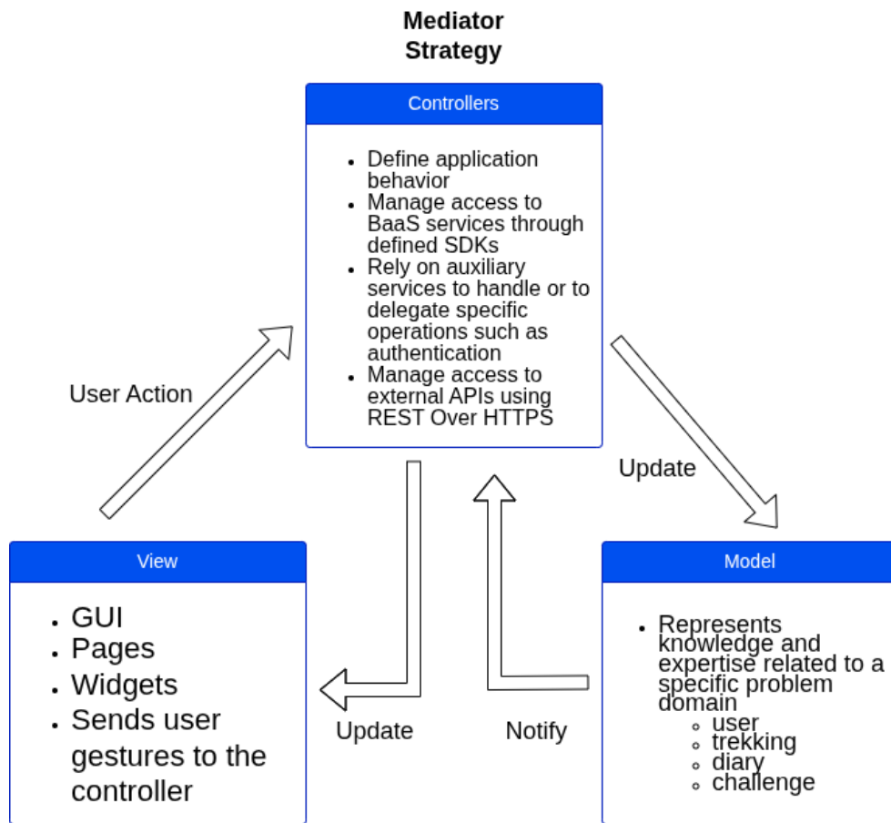
Figure 2.13: Model view controller pattern, adapted from Apple and Oracle documentation
