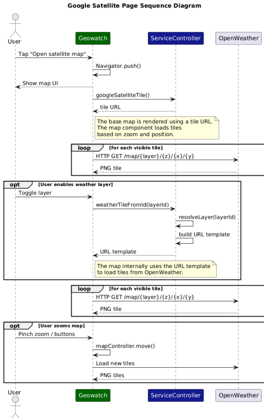
Figure 2.7: View Satellite Weather Information sequence diagram
