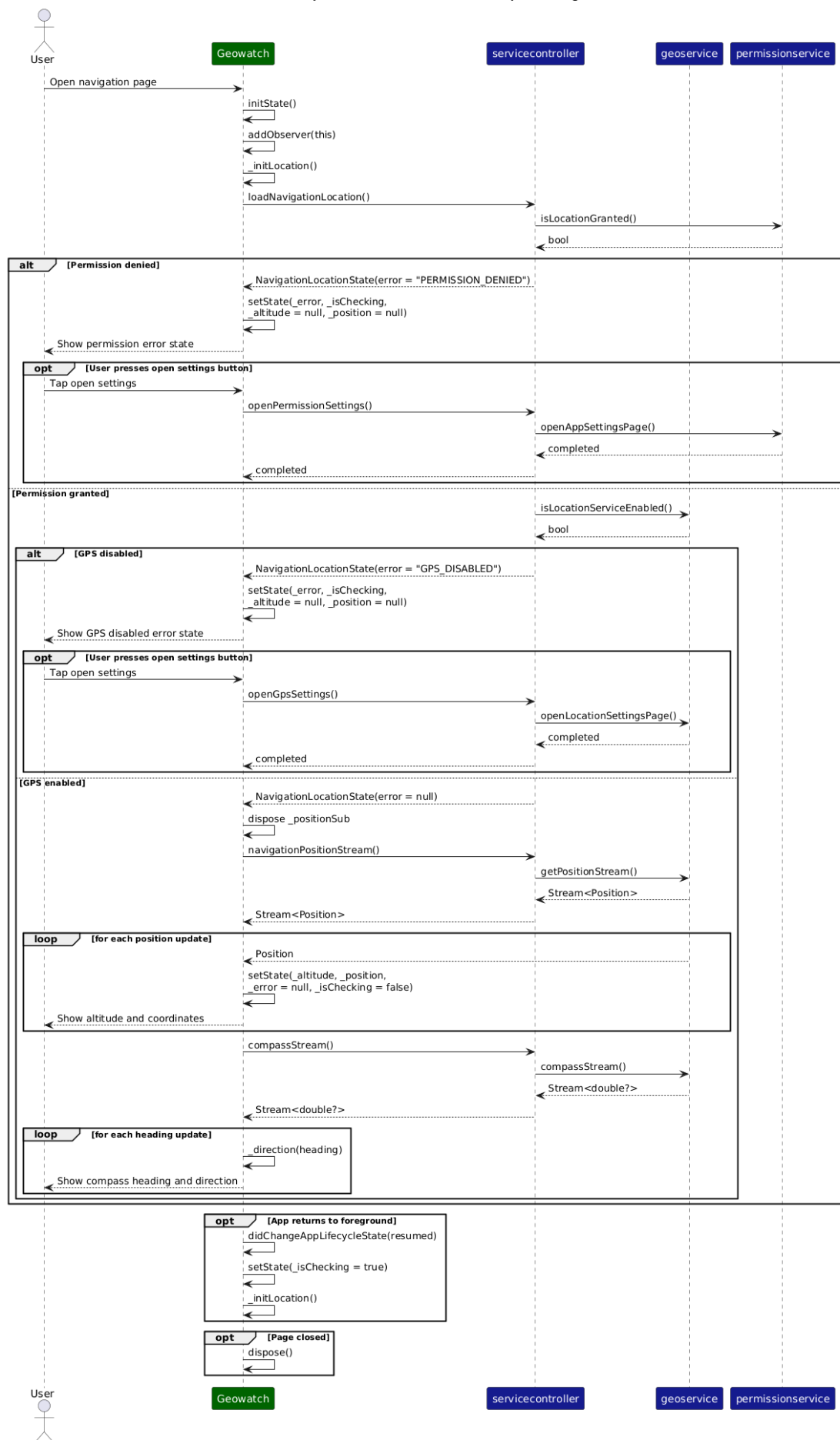
View Compass and Altitude Information Sequence Diagram
